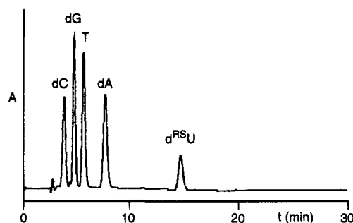
Figure 2. HPLC of enzymatic digestion of d(GACTCT RS 4UTT S 4GAC) (R = CH 3 , 14 ). Detector at 254 nm initially, then 332 nm at 9 min, and 308 nm at 14 min. Ratio of dC/dG/T/dA/d RS 4U (3/2/4/2/1) was measured as 3.3:2.0:4.1:1.9:1.0.
