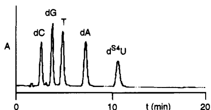
Figure 1. HPLC of enzymatic digestion of d(GACTCT S 4UTT S 4GAC) ( 3 ) into constituent deoxyribonucleosides. Detector at 254 nm initially and then 332 nm at 9 min. Ratio of dC/dG/T/dA/d S 4U (3/2/4/2/1) was measured as 3.3:2.0:4.1:1.9:1.0.
