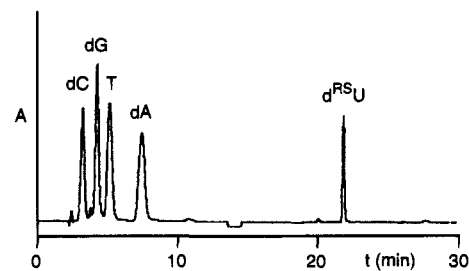
Figure 3. HPLC of enzymatic digestion of d(GACTCT RS 4UTT S 4GAC) (R = SCH 2 CH 2 CH 2 Cl, 16 ). Detector at 254 nm, 332 nm at 9 min, and 308 nm at 14 min. Ratio of dC/dG/T/dA/d RS 4U (3/2/4/2/1) was measured as 3.2:2.0:3.9:1.9:1.1.
